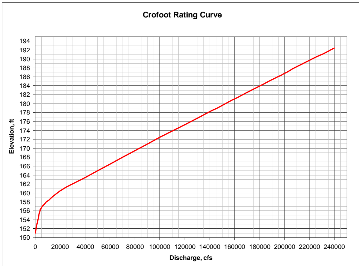
Figure 11. 1921 Rating Curve at Crofoot.
