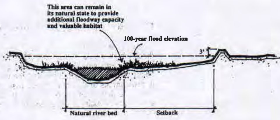
Setback levee.
