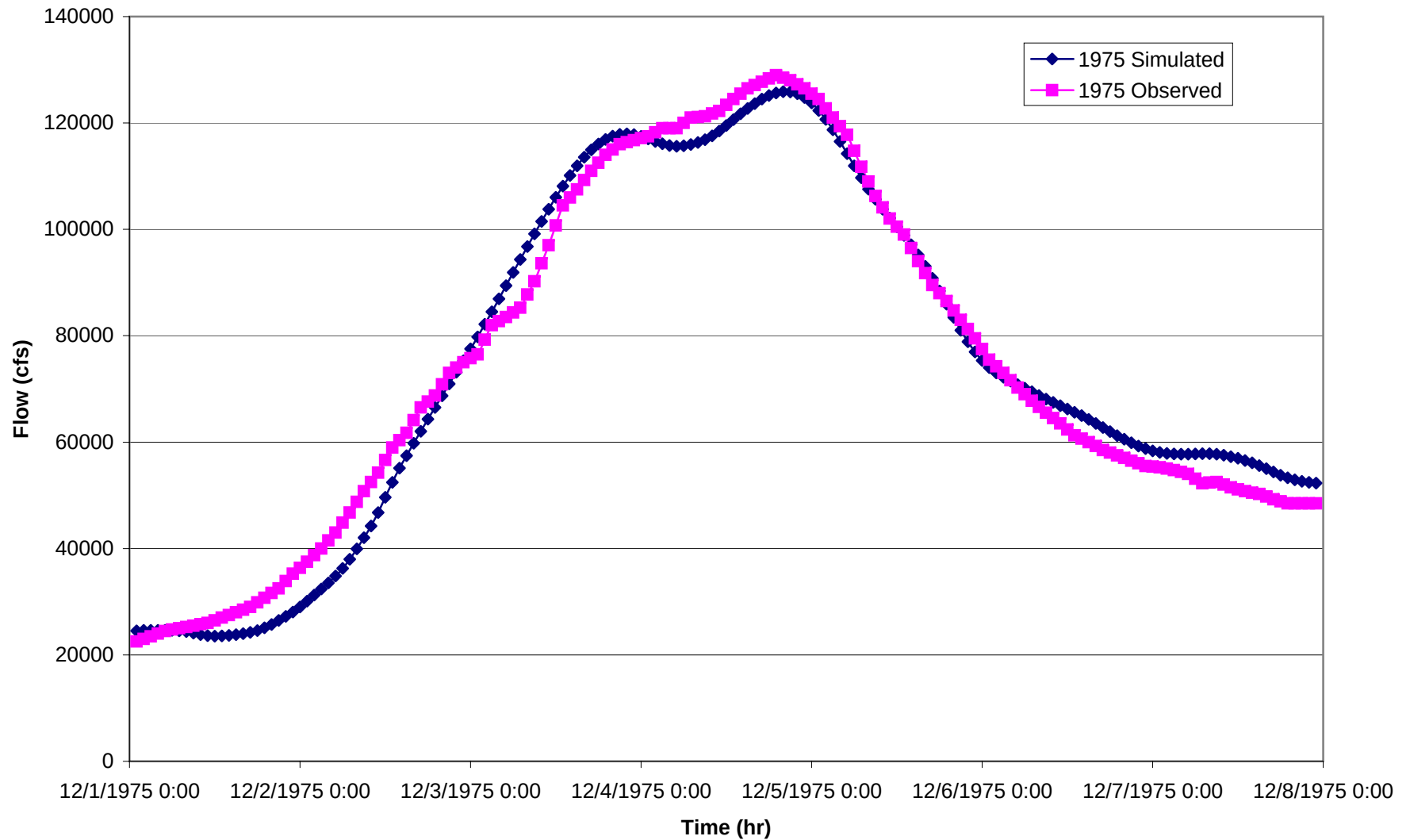
Figure 2 - December 1975 Simulated vs. Observed Hydrograph at Mount Vernon Gage 12A
