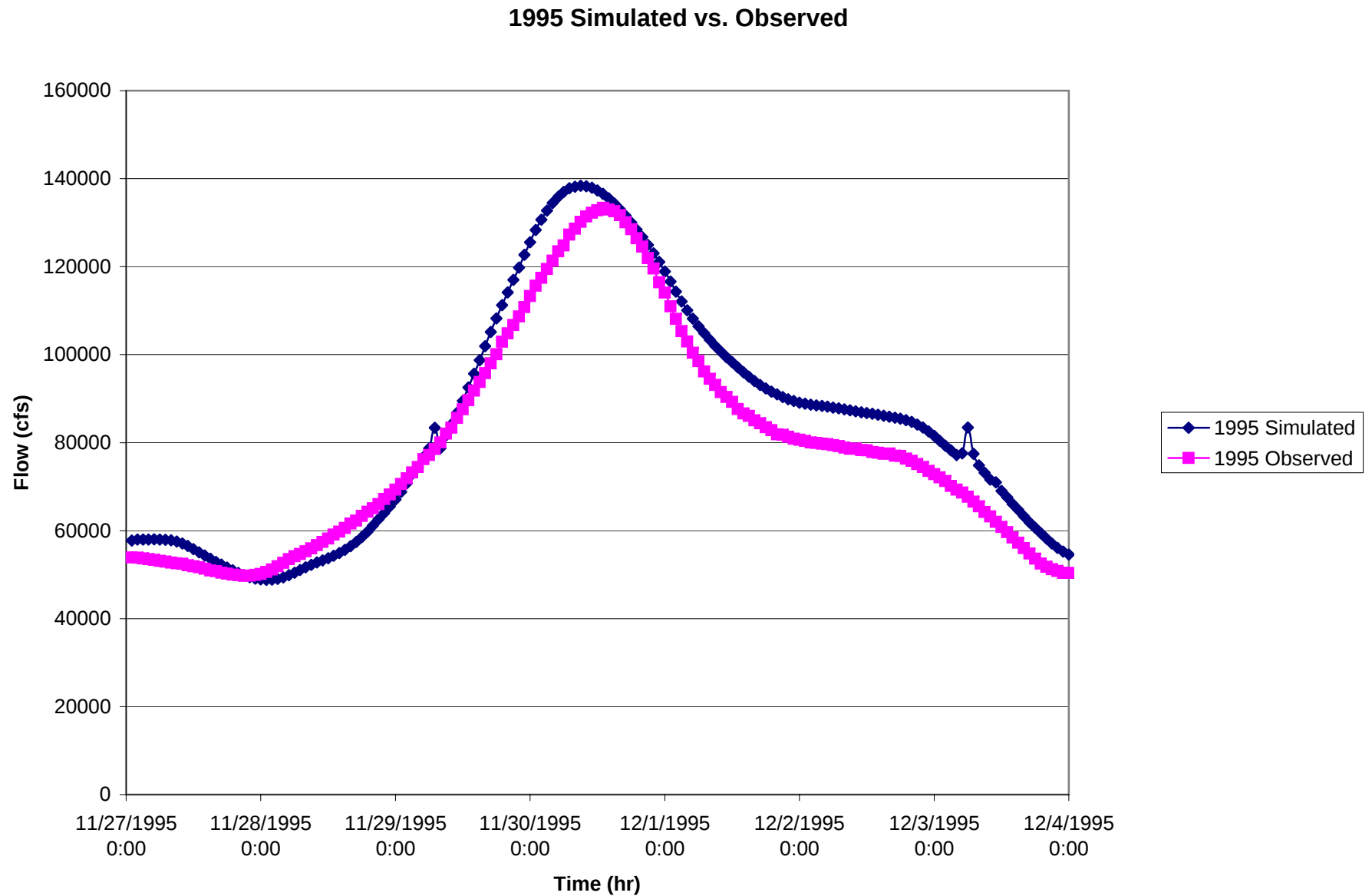
Figure 3 - November/December 1995 Simulated vs. Observed Flow at Mount Vernon Gage 13A
